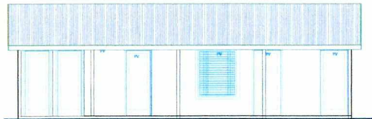
FRONT ELEVATION 01
